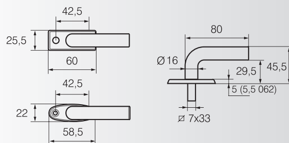
Messinkipainike
